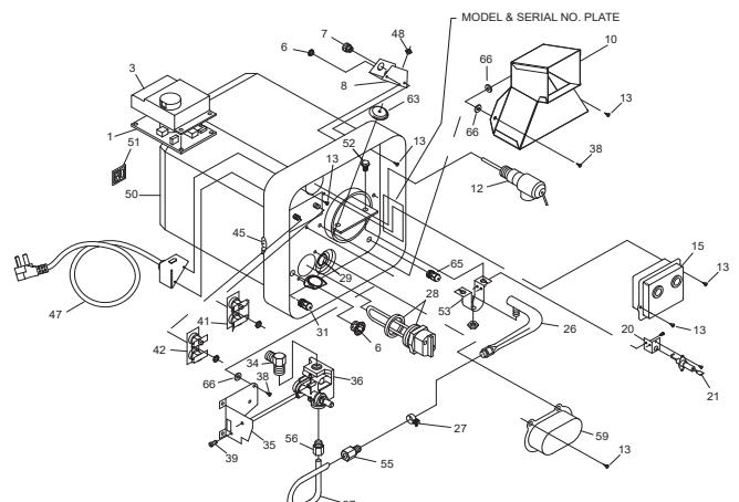
Figure 12 SW4DERA AND SW6DERA SW4DEFA AND SW6DEFA
