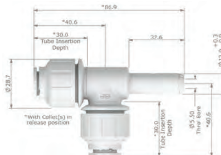
800-02208 JG WATERMARK STEM TEE 12MM PEM5312W
