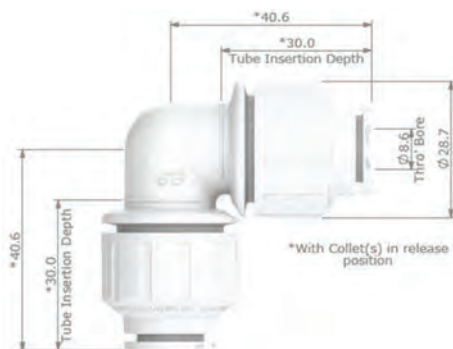
800-02202 JG WATERMARK EQUAL ELBOW 12MM PEM0312W
